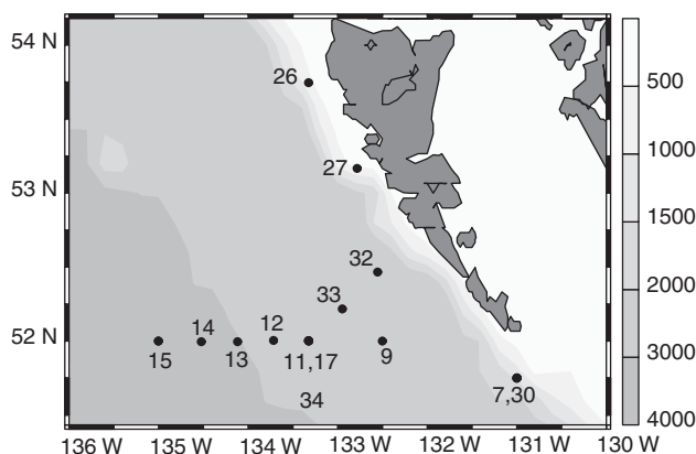
Figure 4 Northeast Pacific sample collection sites used in this study. Shading on the plot indicates bottom depth. Plot was generated using Ocean Data View (Schlitzer, 2012).
