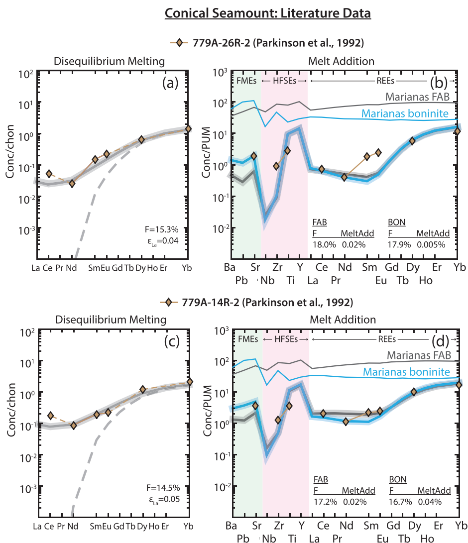
Fig. 11. Disequilibrium melting and melt addition results for clinopyroxene in harzburgites from the Conical Seamount in the Marianas (data from Parkinson et al. , 1992). (a) Disequilibrium melting model results for sample 779A-26R-2. The sample is well matched by \sim 15\% fractional melting at \epsilon_{La} = 0.04 . (b) Melt addition model results for sample 779A-26R-2, comparing the effects of adding a boninitic melt versus a basaltic melt. Both melt compositions are from Reagan et al. (2010). Either of the two melts can match the HREE and LREE, whereas only the boninitic melt matches Sr, and neither melt matches Zr, Ti, and the MREE. (c) Disequilibrium melting model results for sample 779A-14R-2. The sample is well matched by 14.5% fractional melting at \epsilon_{La} = 0.05 . (d) Melt addition model results for sample 779A-14R-2, comparing the effects of adding the same boninitic and basaltic melts as in (b). The sample is well matched by addition of either melt for REE and Sr, but poorly matched for Zr and Ti.
