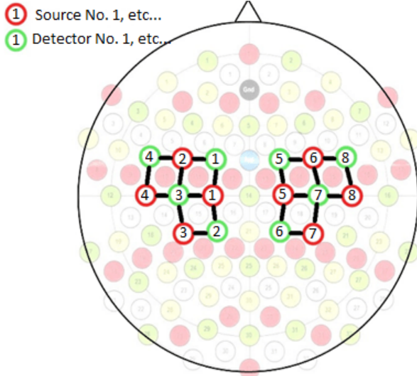
Fig. 3: Montage of the optodes on the head, providing 20 channels of fNIRS data.
