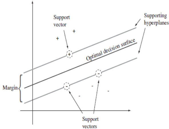
Fig. 6: A concept of SVM and the terms of decision surface, supporting hyperplane and margins.
