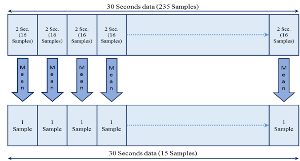
Fig. 5: Schematic of the approach of segmentation.
