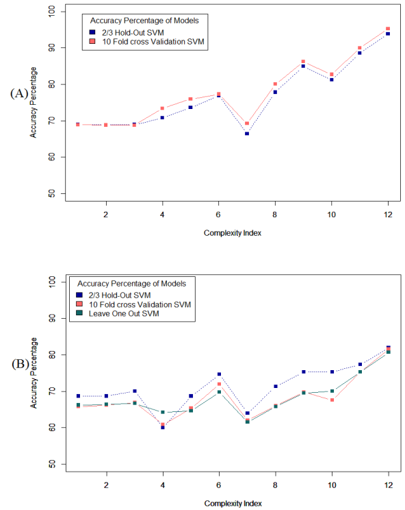
Fig. 7: Accuracy of different methods of classification applied on (A) full length dataset, (B) segmented dataset, on the data recorded from one of the first four participants. Refer to Table II for complexity index.
