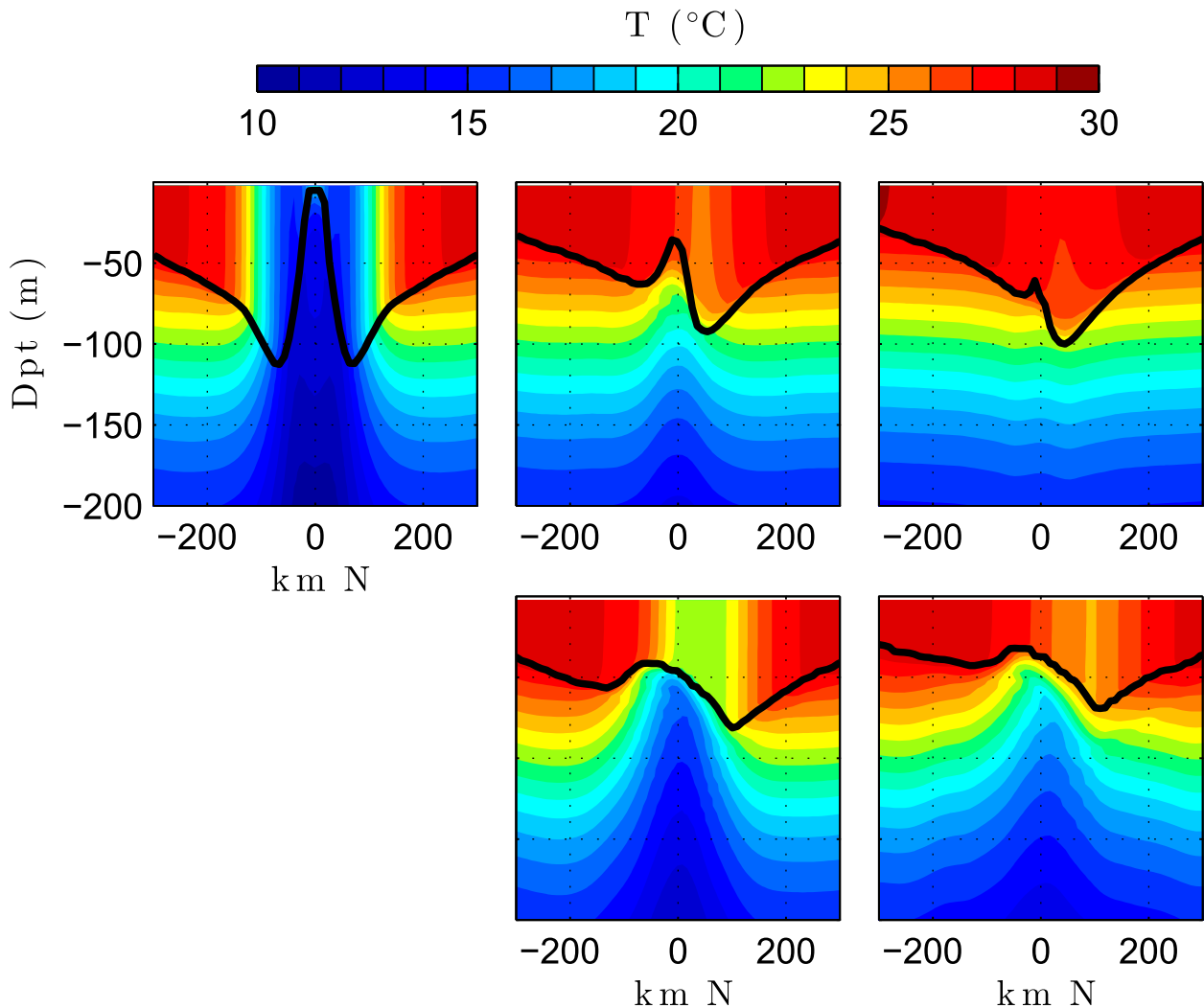
FIG. 3. Vertical transect of temperature in the north–south direction with KPP-ST-noCS. (top) Transects centered at the storm center and (bottom) transects centered at the storm center 18 h prior. The same three storms are presented as in Fig. 1. The thick black line shows the mixing layer depth given by KPP.
