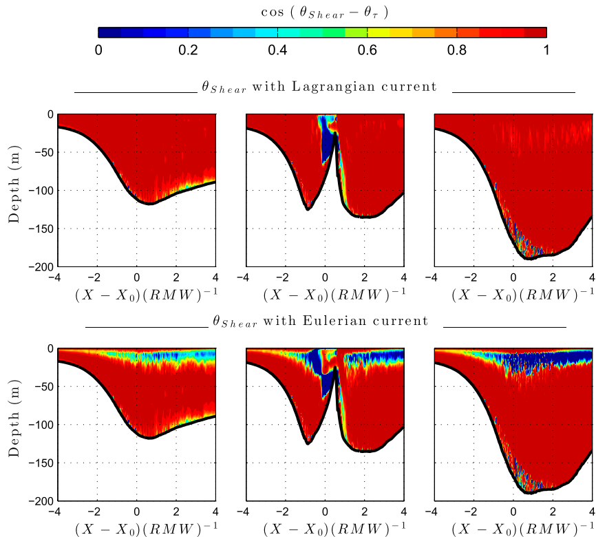
FIG. 4. Cosine of the misalignment angle between the directions of the Reynolds stress \theta_r and vertical gradient \theta_{\partial U_y/\partial z} of the (top) Lagrangian current and (bottom) Eulerian current for 5 \text{ m s}^{-1} , translating tropical cyclone from the LES–LT simulations. The test sites are from (left) 60 km to the left, (center) the storm center, and (right) 50 km to the right. The horizontal axis indicates the distance from the storm center position normalized by the RMW (50 km). Note that the color scale saturates at 0, but negative values can exist within the RMW. The solid black line represents the mixing layer depth using the bulk Richardson number criterion. Values beneath the mixing layer have been filtered out.
