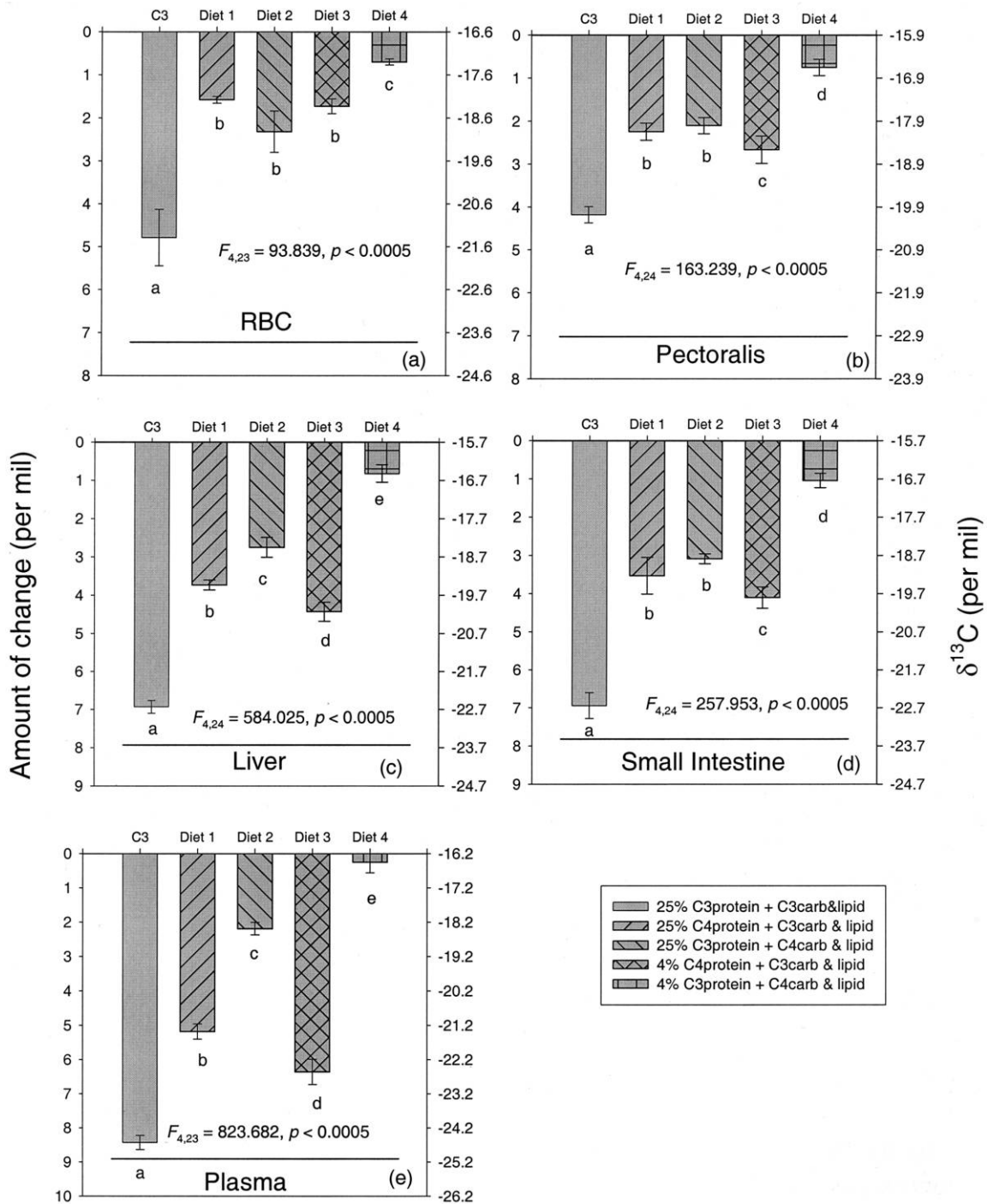
Figure 4. Absolute \delta^{13}\text{C} (‰; mean \pm 1 SD; right Y-axis) and relative amount of change in \delta^{13}\text{C} (‰; left Y-axis) in RBC (a), pectoralis (b), liver (c), small intestine (d), and plasma (e) for yellow-rumped warblers fed the C 4 acclimation diet for 2.5 mo and then switched for 15 d to either the C 3 diet or diets 1–4. X-axis in each panel intersects the Y-axis at the mean \delta^{13}\text{C} (‰) for birds fed the C 4 acclimation diet for 2.5 mo. Solid horizontal line is the mean \delta^{13}\text{C} (‰) for birds fed the C 3 acclimation diet for 2.5 mo for each tissue; n = 6 birds for all samples, except C 3 ( n = 5 birds) and diet 1; RBC and plasma ( n = 5 birds). Bars with the same letter below are not significantly different (diet treatment: F_{4,23} = 661.323, P < 0.0005 ; tissue: F_{4,92} = 443.637, P < 0.0005 ; diet \times tissue: F_{16,92} = 104.856, P < 0.0005 ).
