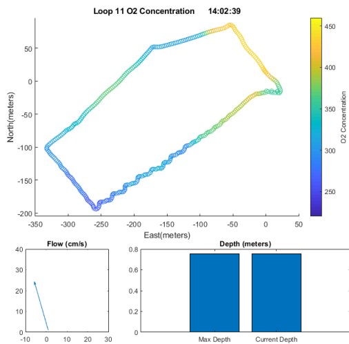
Figure 12 – The dissolved oxygen around the farm using a loop survey
