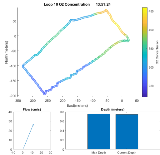
Figure 12 – The dissolved oxygen around the farm using a loop survey
