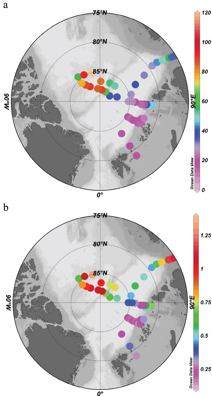
Figure 4. Distribution of (a) ^{228}\text{Ra} ( \text{dpm m}^{-3} ) and (b) ^{228}\text{Ra}/^{226}\text{Ra} ratios in surface waters in summer 2007.
