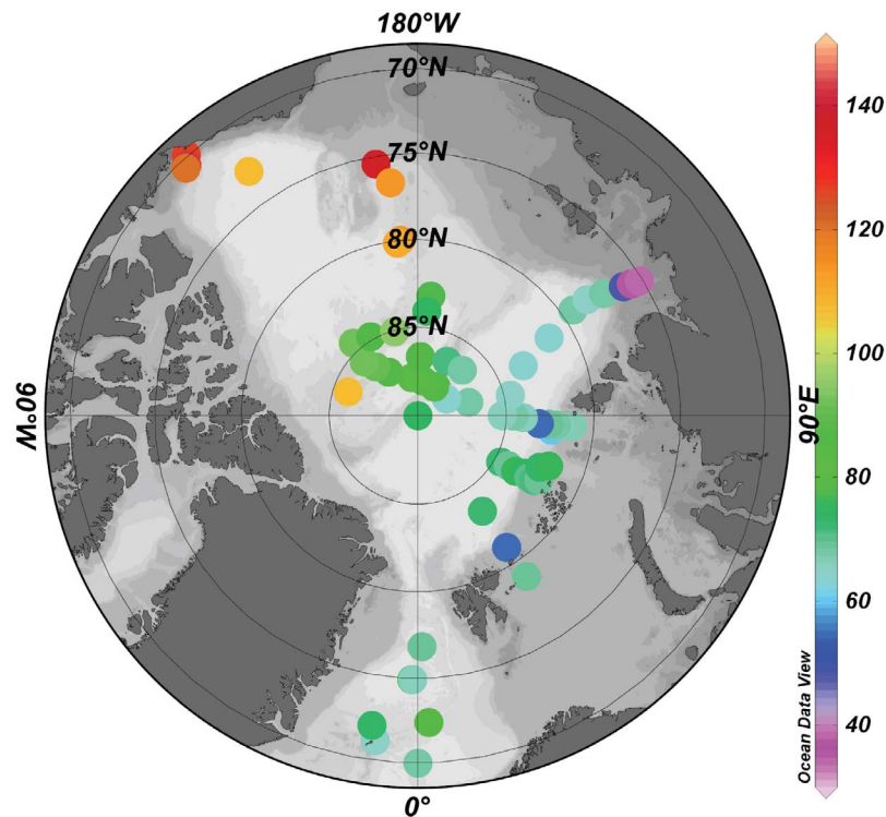
Figure 3. Distribution of ^{226}\text{Ra} ( \text{dpm m}^{-3} ) during ARK XXII/2 compared with literature data (excluding data from the productive Chukchi shelf waters) from GEOSECS Atlantic [Broecker et al. , 1976], Cesar Ice Camp [Moore and Smith, 1986], TTO [Key et al. , 1992], and Smith et al. [2003].
