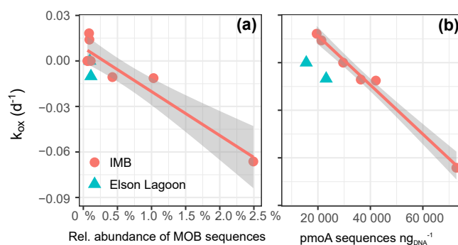
Figure 7. Correlation between net oxidation rate constant ( k_{ox} ) and the relative abundance of sequences in 16S-MOB-OTUs, R^2_{(\text{MOB-OTUs} \sim k_{ox})} = 0.84 (a) and number of pmoA sequences with R^2_{(\text{pmoA} \sim k_{ox})} = 0.85 (b). For correlation to the number of total methylotroph OTUs (which includes MOB and non-MOB methylotrophs in total 16S) R^2_{(\text{Meth-OTUs} \sim k_{ox})} = 0.81 . The gray shaded area shows the 95 % confidence interval of the correlation.
