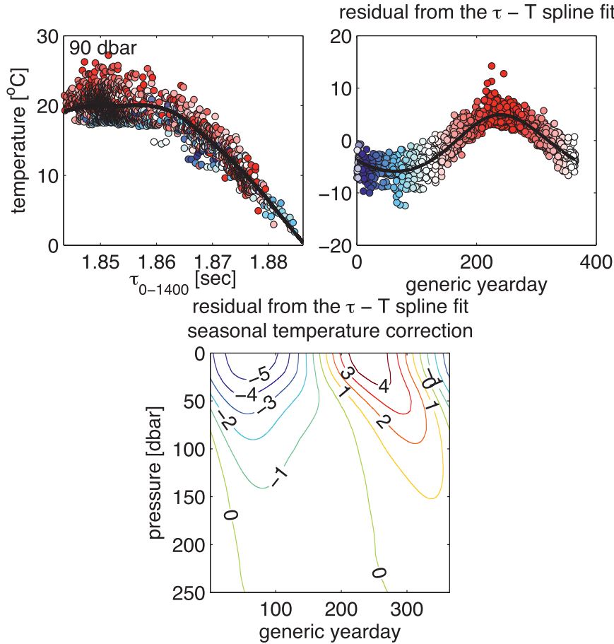
FIG. 15. (top left) Scatterplots of profiling float temperature vs \tau_{index} at 90 dbar with the cubic spline fit shown as a solid dark line. All samples are color coded by generic yearday transitioning from blue in winter to red in summer. (top right) A clear seasonal signal in temperature emerges when the residuals from the spline fit are sorted by time of year. (bottom) Seasonal temperature corrections calculated at 10-dbar increments from the surface to 250 dbar are contoured as a function of yearday and pressure. The temperature seasonal correction ranges through more than 9°C at the surface and decays to less than 0.1°C by 250 dbar.
