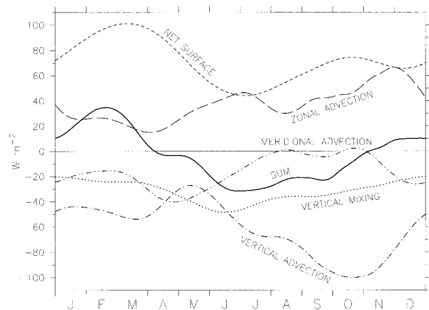
FIG. 11. Terms of the model upper-layer SST balance in the eastern equatorial Pacific (averaged over 2^{\circ}\text{S} – 2^{\circ}\text{N} , 120^{\circ} – 90^{\circ}\text{W} ). Each term is labeled and corresponds to a term in (1). The thick solid line is the sum of all terms (equal to \rho C_p h \partial T / \partial t ).
