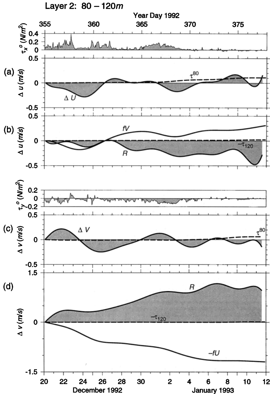
Figure 15. Same as Figure 13, but for layer 2 ( -120 \text{ m} < z < -80 \text{ m} ) and cutoff frequency of 0.25 cpd.
