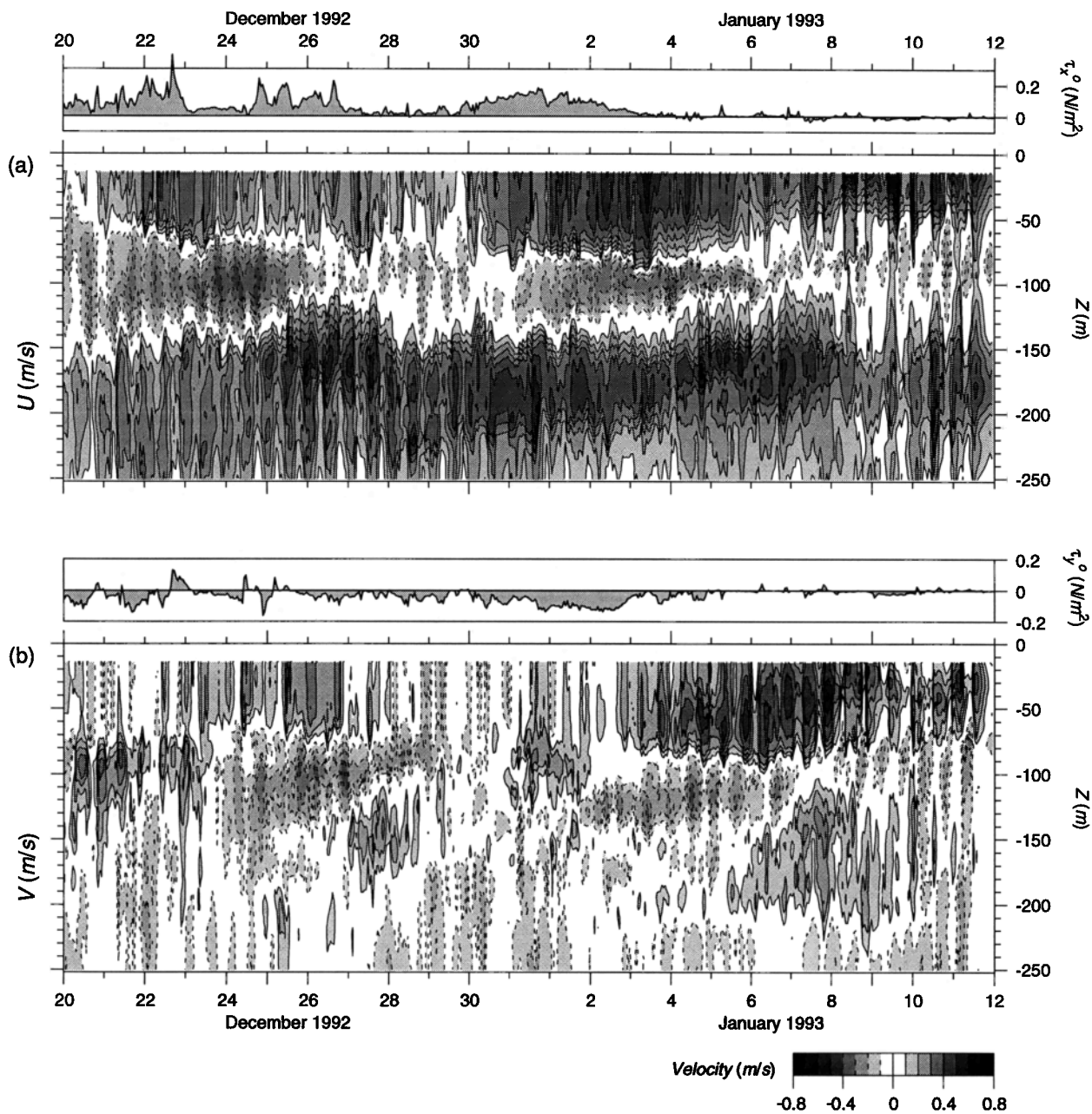
Figure 4. (a) Zonal current. (b) Meridional current. Contours represent \pm 10, \pm 20, \dots \text{cm s}^{-1} . Dashed contours indicate negative values. Current data are from shipboard acoustic Doppler current profilers and are averaged into 1-hour, 4-m bins. For reference, hourly averaged zonal and meridional wind stresses are shown in Figures 4a and 4b (top), respectively.
