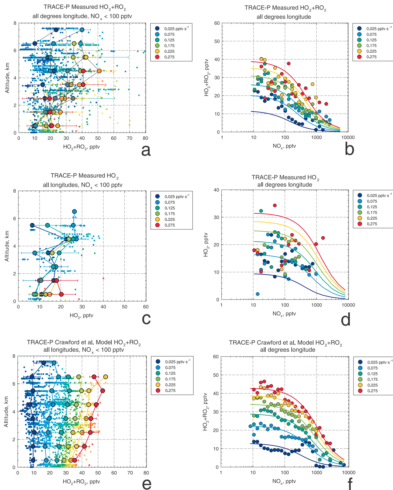
Figure 3. (a) Measured \text{HO}_2 + \text{RO}_2 concentrations versus altitude colored by P_{\text{HO}_x} (pptv \text{s}^{-1} ). Small points are individual 1-min average concentrations, and larger symbols are 1-km altitude bin averages. Data selected for \text{NO}_x less than 100 pptv. (b) Observed \text{HO}_2 + \text{RO}_2 concentrations binned by \text{NO}_x concentration and P_{\text{HO}_x} . Lines are fit to equation (9). (c) Same as Figure 3a for \text{HO}_2 observations. (d) Same as Figure 3b for \text{HO}_2 observations. (e) Same as Figure 3a using results of Crawford et al. [1999] model of TRACE-P observations. (f) Same as Figure 3b using results of Crawford et al. [1999] model.
