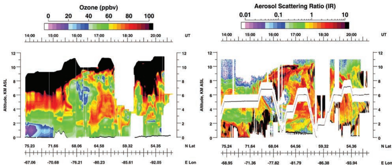
Figure 1. Ozone and aerosol scattering ratio distributions obtained on flight from Thule, Greenland to Winnipeg, Canada on 22 May 2000 (Flight 41). Aircraft flight altitude is shown on the aerosol plot as a continuous black line. In situ O_3 measurements are used to constrain and interpolate the DIAL O_3 data across the near-field range above and below the aircraft (shown as white on aerosol plot) where DIAL measurements are not made.
