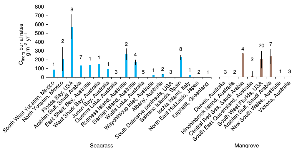
Fig. 3 Inorganic carbon burial rates in all locations. Mean C_{inorg} burial rates in all locations in sediment cores for seagrass meadows and mangrove forests, organized from low to high latitudes. Bars are the SE. Labels are the number of cores per location
