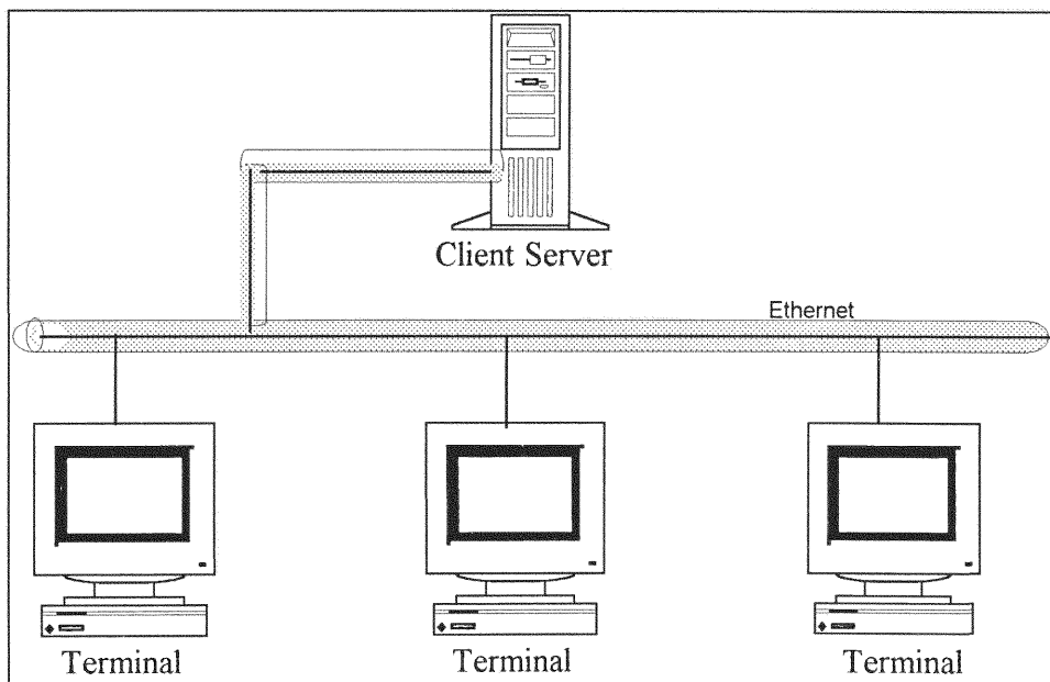
Figure 4.2 Client Server
