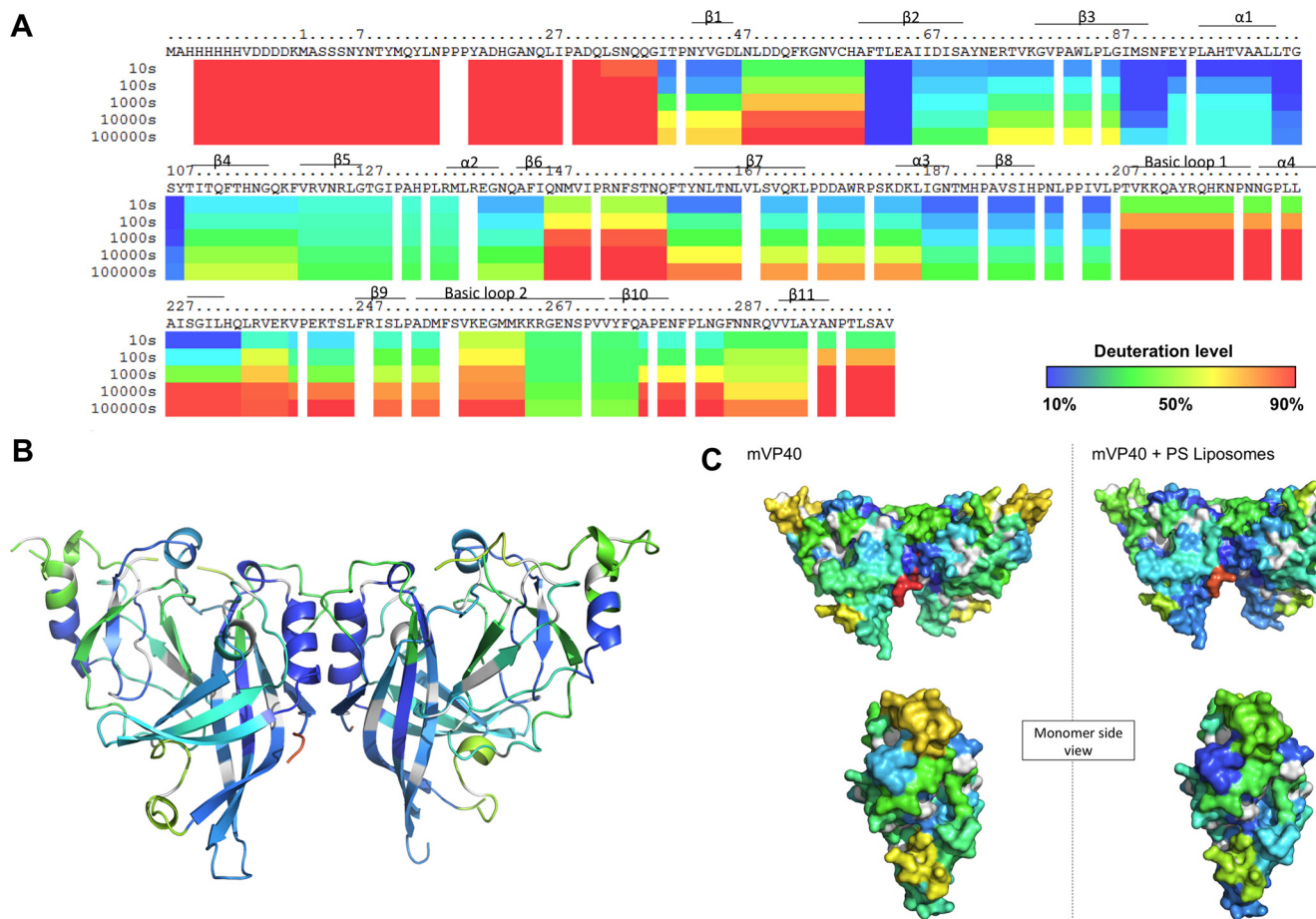
Figure 7. Hydrogen/deuterium exchange of mVP40 in the presence of PS containing vesicles. A , ribbon map indicating the percentage of hydrogen/deuterium exchange that occurred in peptide fragments over the entire exchange period. Each row corresponds to each time point from 10 to 100,000 s. Color coding indicates the percentage of deuterium incorporation in the given time point. B , percent labeling of the 10-s time point mapped onto the crystal structure of mVP40 (PDB code 5B0V). Color coding is as indicated in A . C , space filling models of mVP40 protein ( right ) and mVP40 after incubation with lipids. Side view of a mVP40 monomer is also shown for both conditions.
