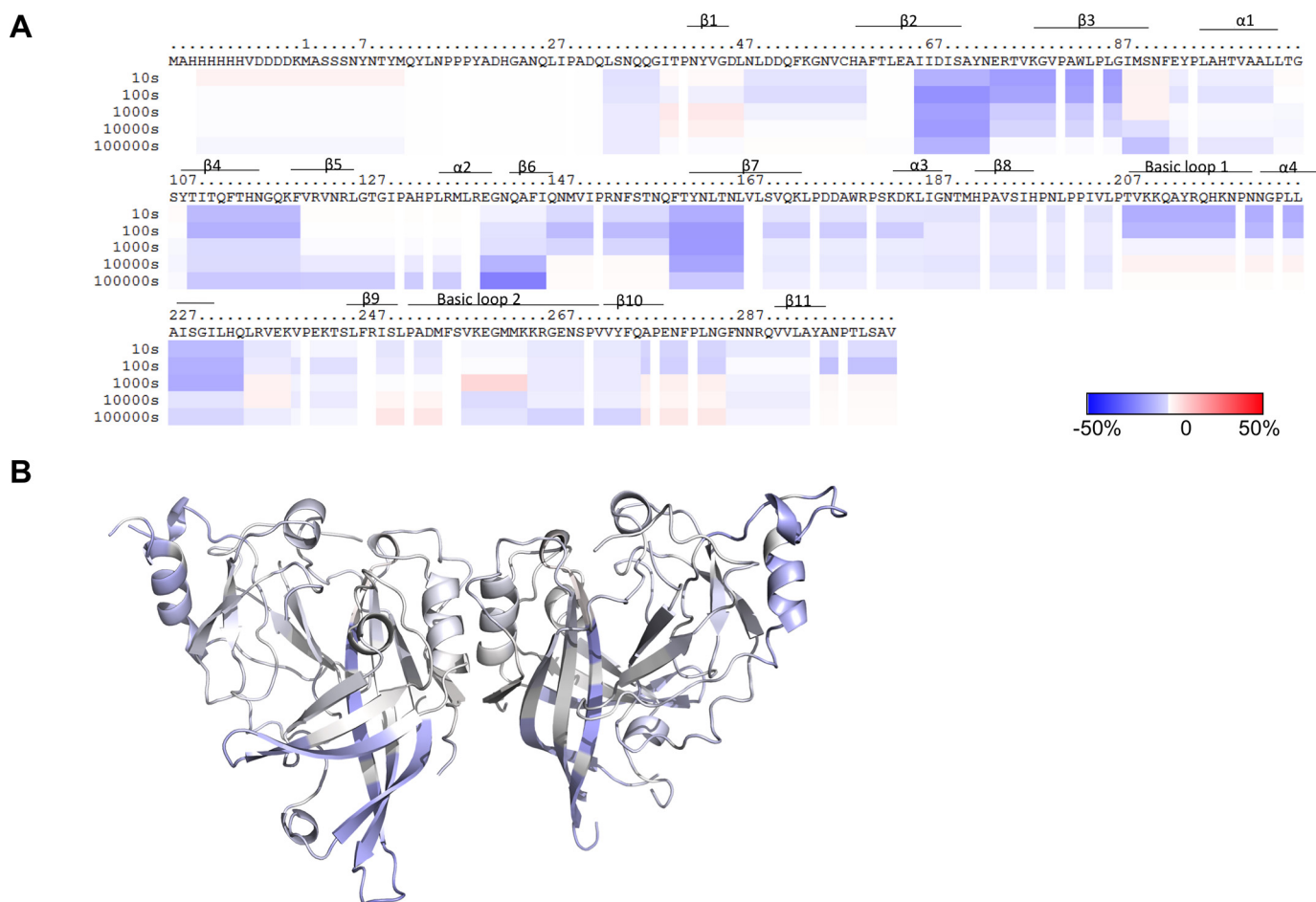
Figure 8. Influence of membrane association on mVP40 as a measure of the change in deuteration level (D%) in comparison to mVP40 in the absence of liposomes. A , difference in deuterium percentage of mVP40 in the presence of liposomes was mapped to the sequence over the entire exchange period. Each row corresponds to each time point from 10 to 100,000 s. Color coding: blue indicates the regions that exchange slower in the presence of lipid and red indicates the regions that exchange faster in the presence of lipid. B , differences in deuteration level (D%) in the presence of liposomes of the 10-s time point mapped on to the crystal structure of the mVP40 (PDB code 5B0V).
