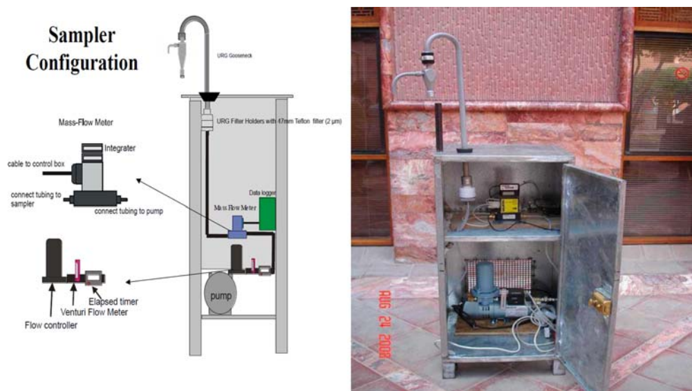
Figure 3. Schematic of the PM_{2.5} sampler (left) and image of sampler used in the study (right).
