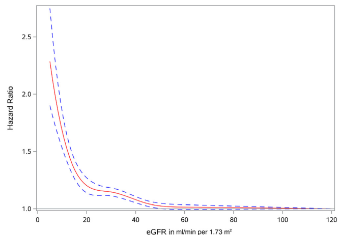
Figure 3 | Spline analysis of the relationship between time-updated estimated glomerular filtration rate (eGFR) and risk of incident diabetes mellitus. The red line represents the hazard ratio, and dashed blue lines represent 95% confidence intervals. eGFR = 120 ml/min per 1.73 m 2 was the reference.
