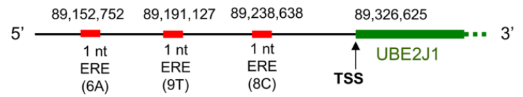
perfect ERE and 1 nt variant EREs in front of UBE2J1 on chromosome 6 for human
