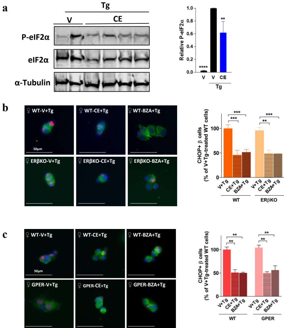
Figure S3. Related to Figure 3. (a) Male Ins2 +Akita \beta -cells were treated with the indicated compounds for 24h followed by exposure to Tg for 4h. Representative Western blot for elf2 \alpha protein phosphorylation and total protein (left) and relative elf2 \alpha phosphorylation/total protein levels quantified by densitometry (right) are shown (n=4 experiments). (b) Dispersed islets from female WT, ER \beta KO and (c) GPERKO mice were treated with the indicated compounds for 24h followed by exposure to Tg for 4h. Representative images of immunofluorescent staining for CHOP (red), insulin (green) and nuclei (blue) and quantification of \beta -cells with CHOP + nuclei relative to vehicle are shown (n=3 experiments). Data are shown as mean \pm SEM. **P < 0.01, ***P < 0.001.
