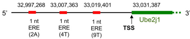
perfect ERE and 1 nt variant EREs in front of UBE2J1 on chromosome 4 for mouse
