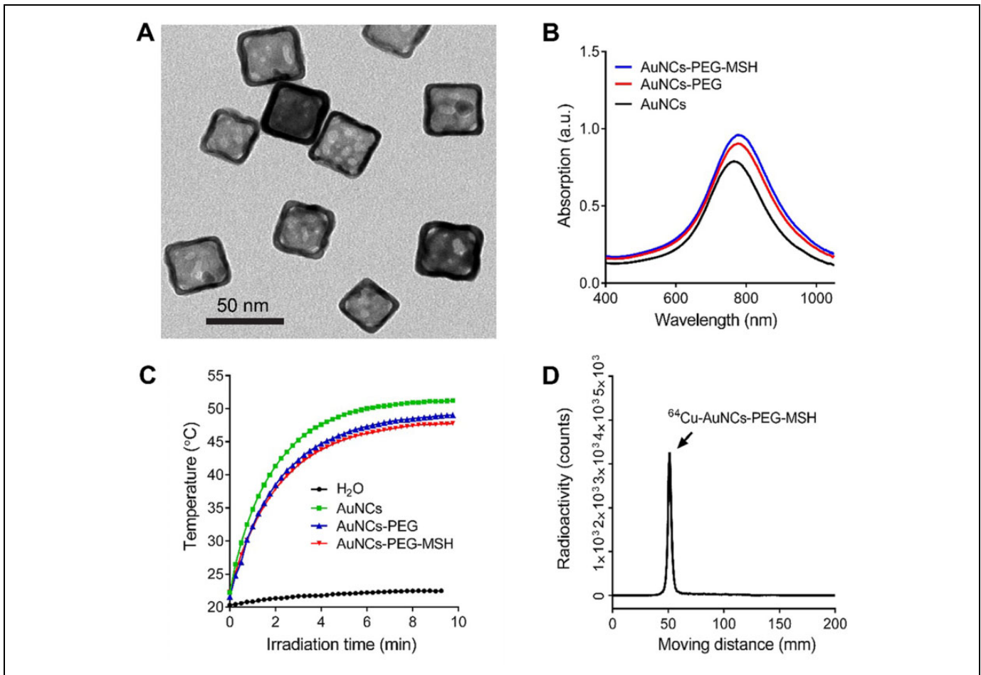
Figure 2. Characterization of gold nanocages. A, Transmission electron microscopy image of AuNC-PEG-MSH. B, UV-Vis spectra of unmodified gold nanocages (AuNCs), AuNCs-PEG, and AuNCs-PEG-MSH showing similar LSPR peaks. C, Plots of temperatures as a function of irradiation time for suspension of H 2 O, AuNCs, AuNCs-PEG, AuNCs-PEG-MSH. The concentration (0.025 nmol/L) of each suspension had the same maximum extinction intensity. The laser power density was 1.1 W/cm 2 . D, Instant radio-thin layer chromatogram (iTLC) of purified 64 Cu-AuNCs-PEG-MSH.
