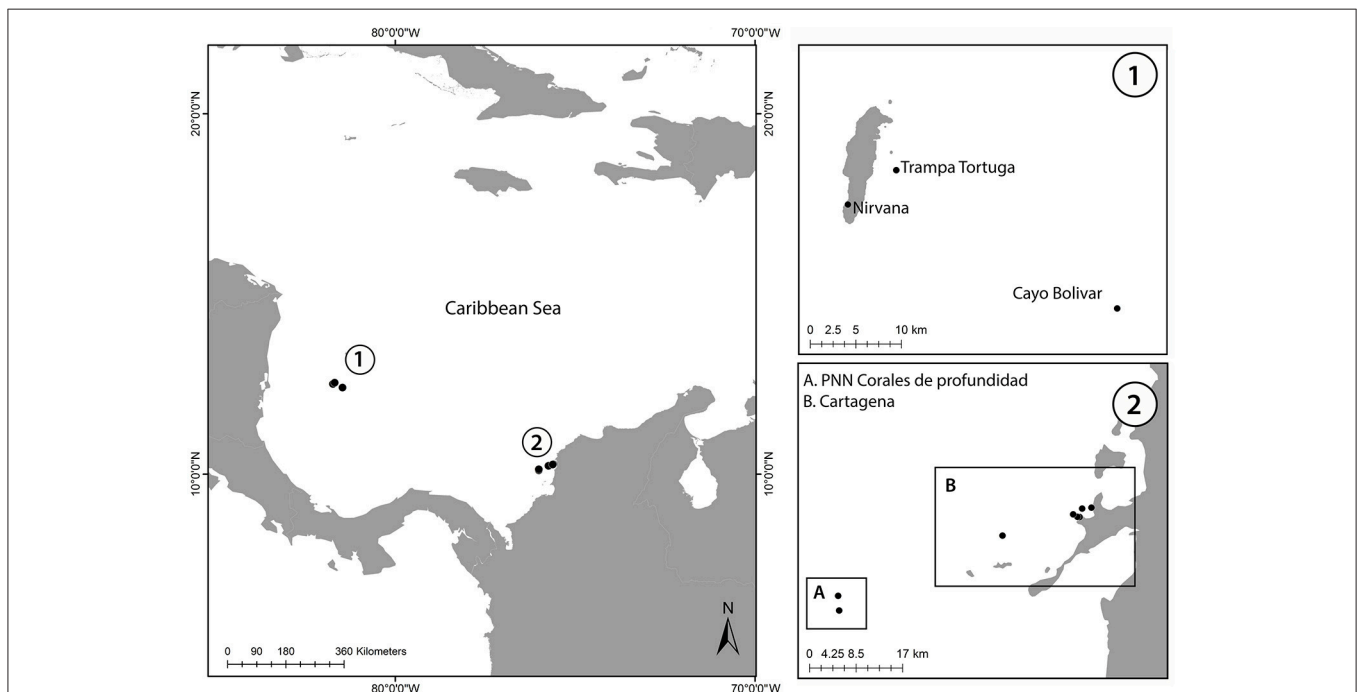
FIGURE 1 | Map of the sampled locations in Colombian Caribbean. (1) Map of San Andrés Island showing the three localities where colonies were sampled. (2) Caribbean coast of Colombia showing the two localities (A) Parque Nacional Natural Corales de Profundidad (B) Cartagena Bay.
