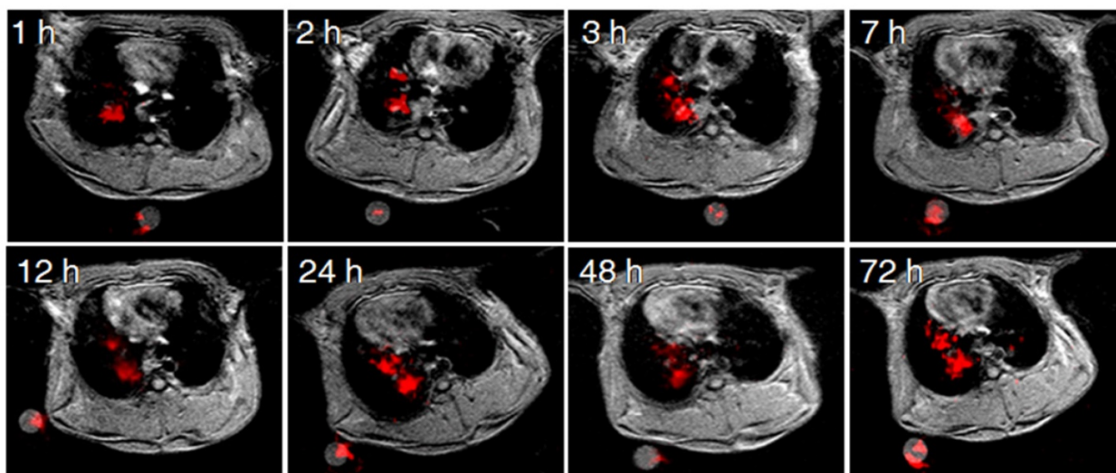
Figure 3. Dynamic monitoring of 19 F-MR enhancement at different time points post IT delivery of the M-PFC NPs. Image slices were acquired at different time points and examples selected to depict similar cardiothoracic regions.
