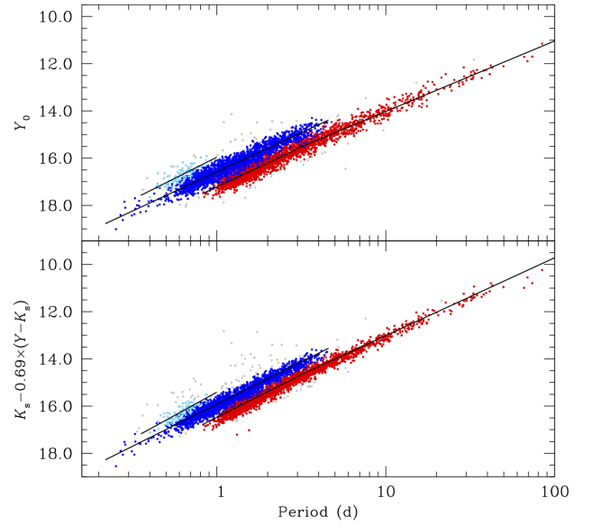
Figure 4. PL(Y) and PW(K_s, Y) relations for the SMC CCs investigated in this paper. F, 1O and 2O pulsators are shown as red, blue and light blue filled circles, respectively. The grey filled circles show objects excluded from the analysis because they deviate more than 3.5\sigma from the best-fits to the data represented by solid lines.
