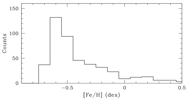
Figure 10. Distribution of the individual photometric metallicities for the CCs analysed in this work. Note that the absolute [Fe/H] values can be overestimated by \sim 0.1 dex (see text).
