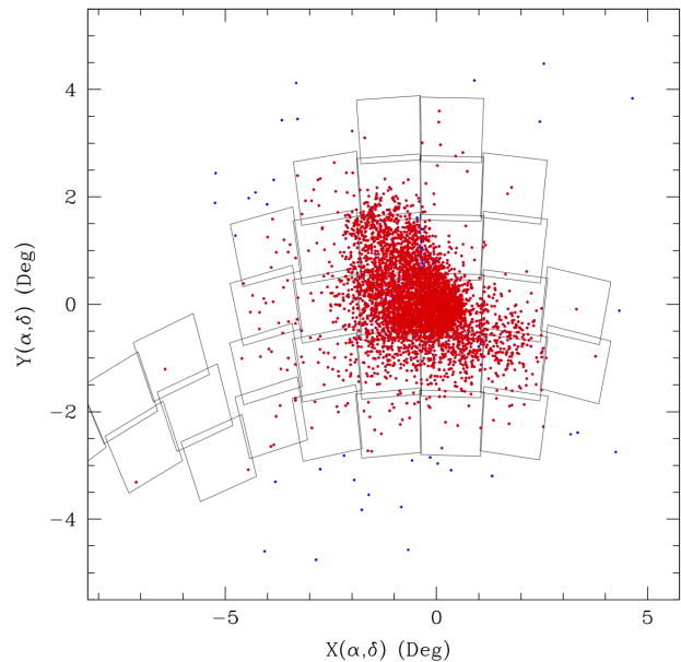
Figure 1. Map of the CCs in the SMC. Red and blue circles show CCs in the OGLEIV survey with and without counterparts in the VMC survey, respectively. The solid rectangles show the location of the VMC tiles. The centre is at \alpha_0=12.54 deg; \delta_0 = -73.11 deg.
