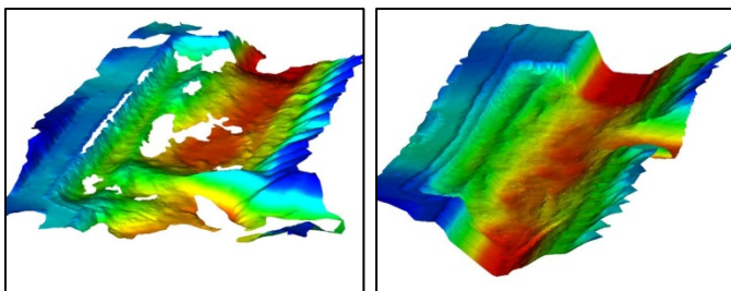
Figure 3. Data Sets from Laser Scanning (left) and UAS (right).
