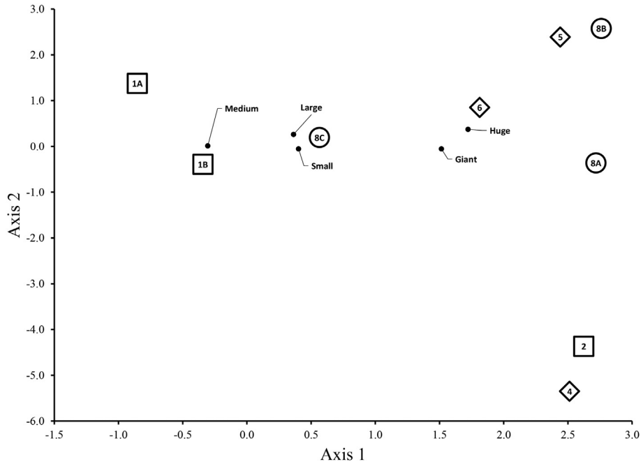
Figure 7. Correspondence analysis of murine body size abundances within stratigraphic units. Axes 1 and 2 represent 95.7% and 2.7% of the variance, respectively. Unit symbols: >50 ka, squares; 50 to 12 ka, diamonds; 12 ka to present, circles.
