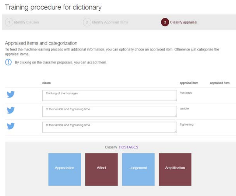
Figure 2. Classifying Appraisal Items
