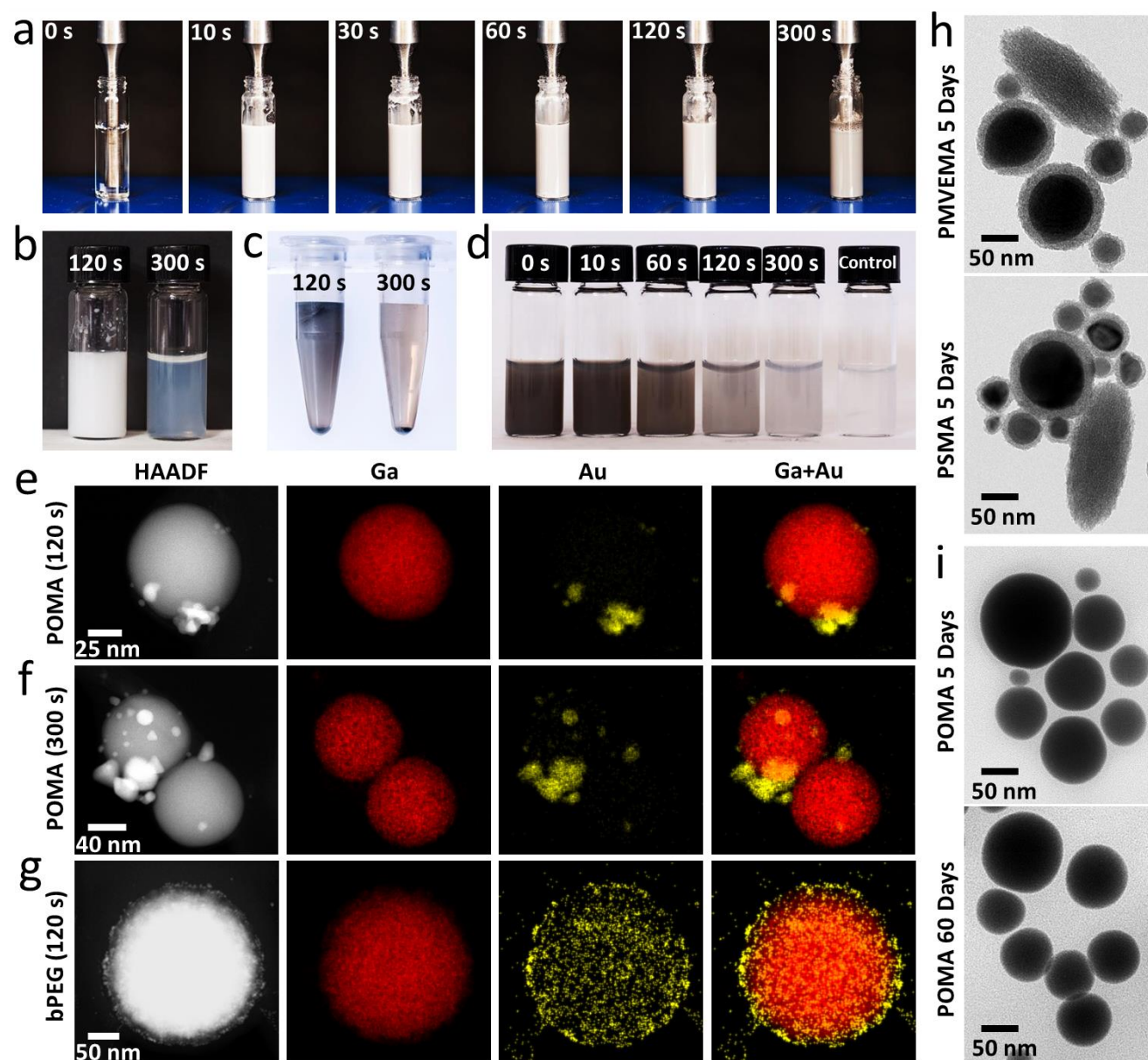
Figure 2. Investigating the mechanism behind the production of POMA grafted EGaIn NPs. (a) Sequential snap shots showing the NP suspension during the production process. (b) Water-POMA-toluene mix 120 and 300 s after activating the sonication probe. (c) Centrifuged LM NP suspension 120 and 300 s after activating the sonication probe. (d) Image of the supernatants for LM NPs produced with different pre-sonicating time; the control sample lacks EGaIn during sonication. TEM image and EDS mapping of the POMA grafted EGaIn NPs produced with (e) 120, and (f) 300 s sonicating time after galvanic replacement reaction. (g) TEM image and EDS mapping of the bPEG-grafted EGaIn NPs after galvanic replacement reaction. (h) TEM images for PMVEMA and PSMA grafted LM NPs 5 days after production. (i) TEM images for POMA grafted LM NPs 5 and 60 days after production.
