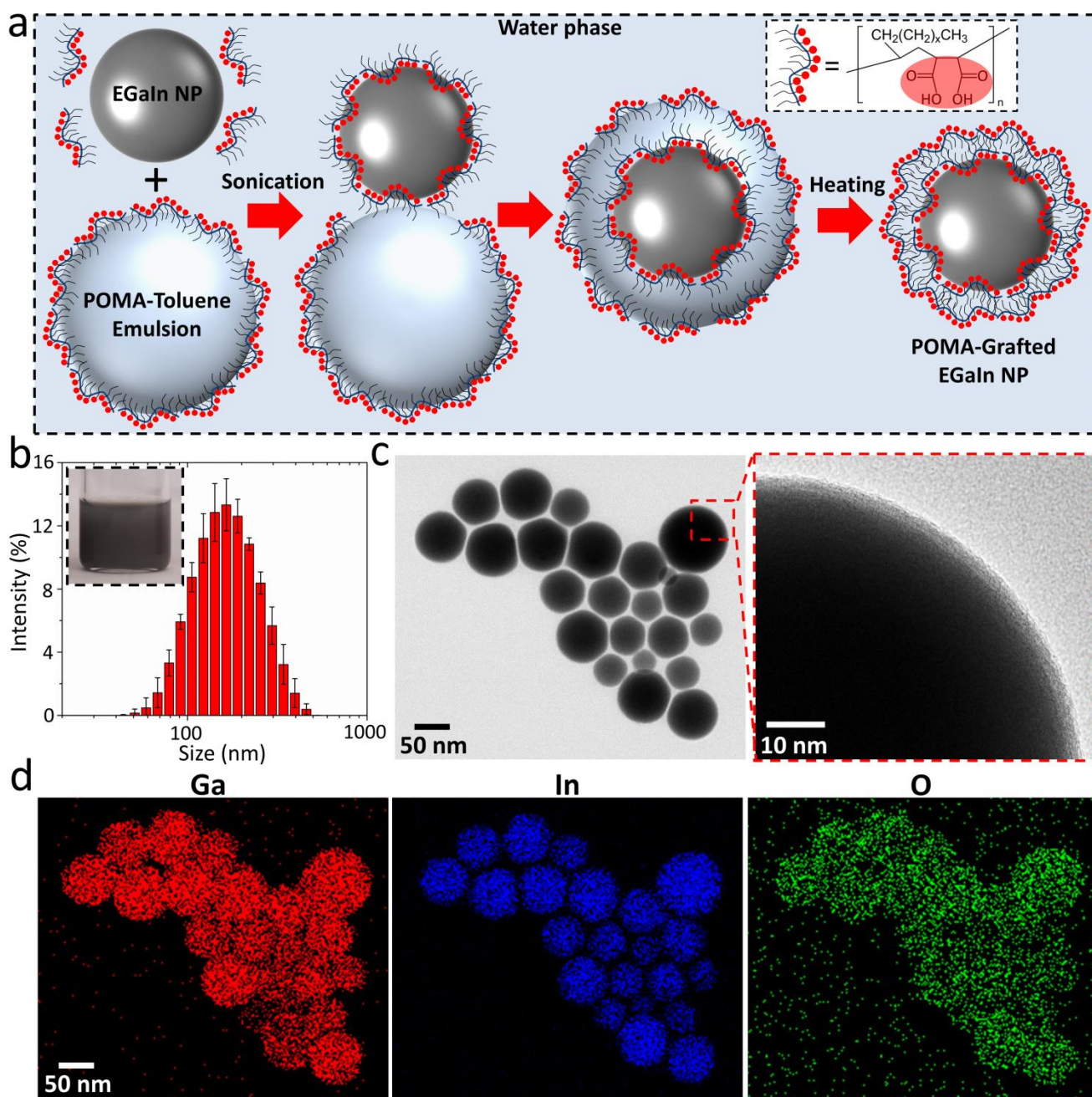
Figure 1. Production of POMA grafted EGaIn NPs. (a) Schematic depicting the mechanism leading to the production of stable liquid metal NPs. (b) Hydrodynamic size distribution of the POMA grafted EGaIn NPs; the inset shows the NP colloidal suspension. (c) TEM images of the produced NPs. (d) EDS mapping of gallium, indium, and oxygen for the NPs.
