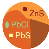
Pb-sulfides, Pb-chlorides & sphalerite enclosed in magmatic sulfide blebs
