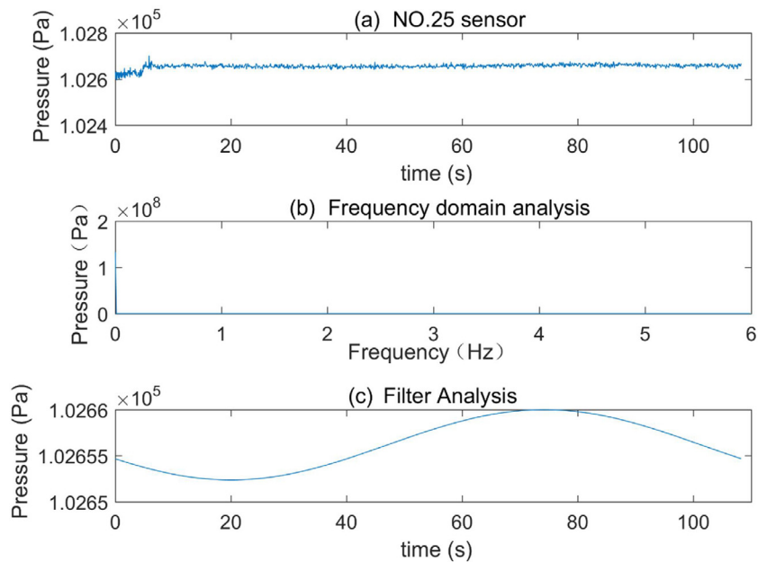
Figure 15. The process of sensor No. 25 pressure data.
