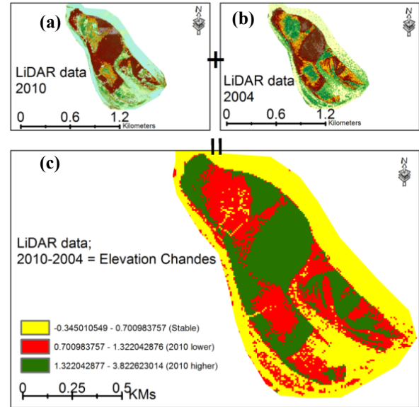
Fig. 2 The temporal differential of the case study elevation shows; (a) LiDAR based DEM of 2010, (b) LiDAR-based DEM of 2004, and (c) elevation changes over the 6-year period, red is loss, green is accretion, stable parts are yellow
