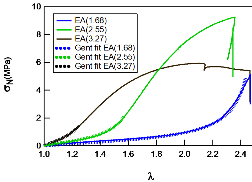
Figure S2: Stress-strain curves of different multiple networks (value of \lambda_0 shown in the legend) to illustrate the typical quality of the fit by Gent's model. \dot{\lambda} = 0.021 \text{ s}^{-1}
