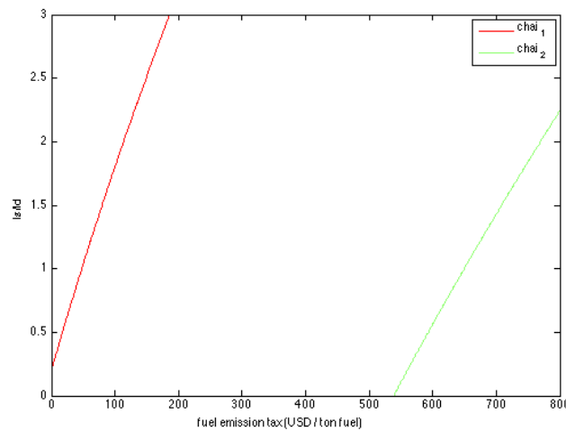
Figure 6. Values of threshold \chi_1 and \chi_2 for different l_s / l_d and fuel emission \chi
