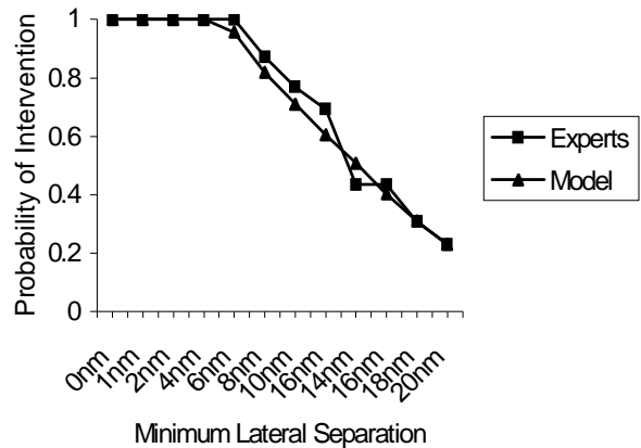
Figure 2. The probability of intervention by experts and the predictions of model.
