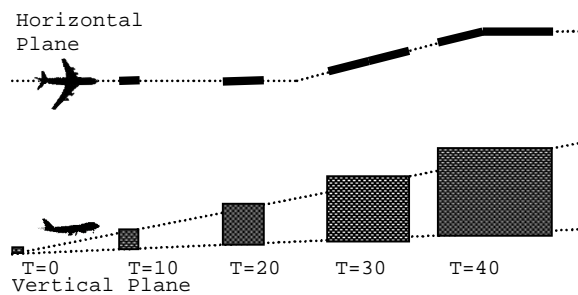
Figure 1. Modeling position uncertainties (adapted from Granger et al, 2001, figure 3). The location of an aircraft projected into the future is bounded by its best and worst case flight performance, with a potential conflict being detected if the regions of two aircraft violate separation standards.
