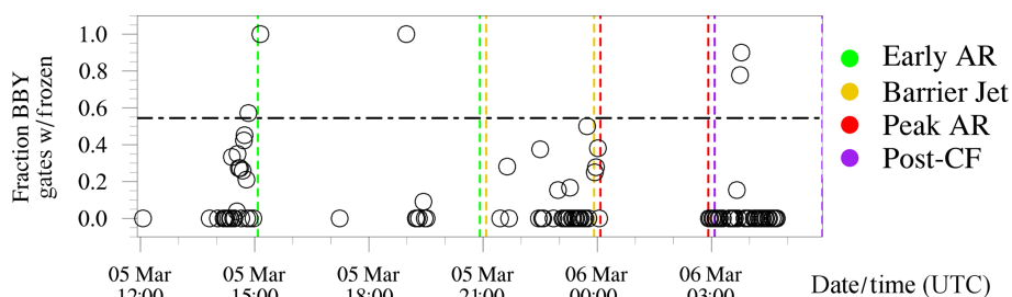
Figure 7. (a) Time series of P_{\text{frz}}^{\text{BBY}} (black circles) in the unblocked layer from all KDAX scans detecting precipitation at the BBY azimuth. The all-storm mean of P_{\text{frz}}^{\text{CZC}} is shown by the horizontal dot–dash black line. Vertical dashed lines show the boundaries of kinematic periods, as coded by color in the legend.
