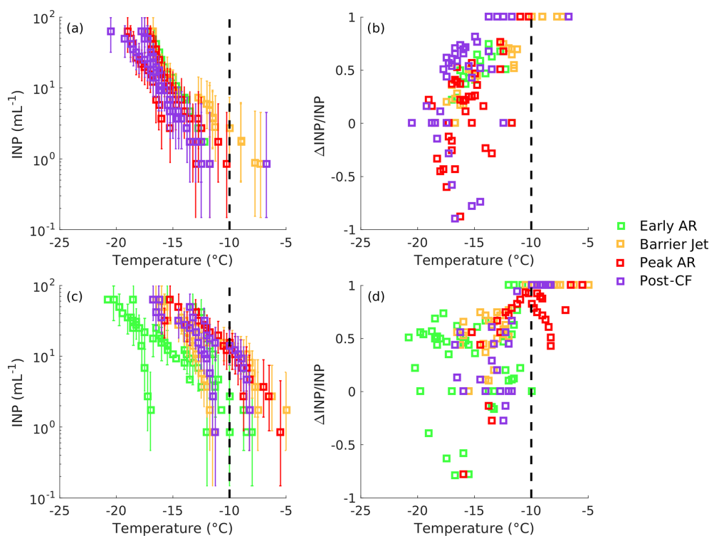
Figure 5. (a) Unheated \text{INP}(T) ( \text{mL}^{-1} ) from BBY precipitation during Early AR (green), Barrier Jet (yellow), Peak AR (red), and Post-CF (purple) periods. Whiskers denote technique standard error ( \text{mL}^{-1} ). (b) As in a, except for \Delta\text{INP}(T)/\text{INP}(T) . (c) As in (a), except for unheated precipitation samples from CZC. (d) As in (c), except for \Delta\text{INP}(T)/\text{INP}(T) .
