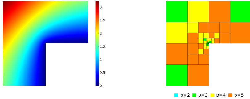
FIGURE 5.6. Left: The DPG* solution v . (Color scale represents solution values.) Right: The corresponding hp quadtree mesh found by the hp -adaptive algorithm after fifteen refinements. (Colors represent polynomial degrees p .)
