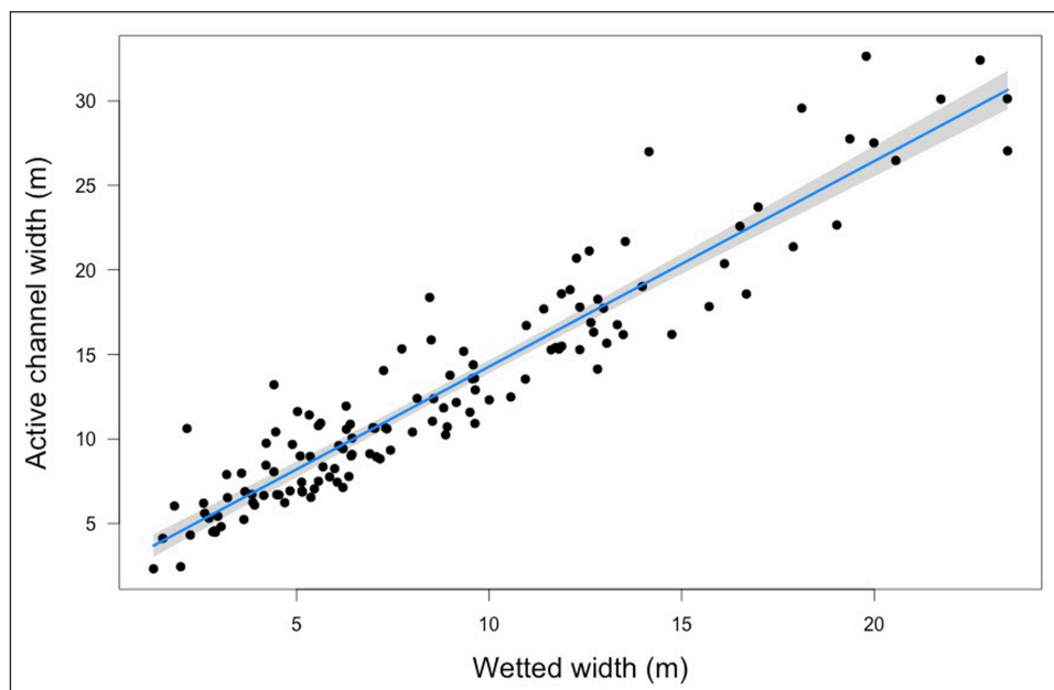
Figure 3: Relationship between active versus wetted stream width. Linear relationship between active ( W_p ) versus wetted ( W_w ) stream channel widths from contemporary Aquatic Inventory Program stream surveys ( W_A = 2.12 + 1.22 \times W_w , n = 131 , R^2 = 0.89 , p < 0.001 ). Shaded area represents 95% confidence band. DOI: https://doi.org/10.1525/elementa.192.f3
