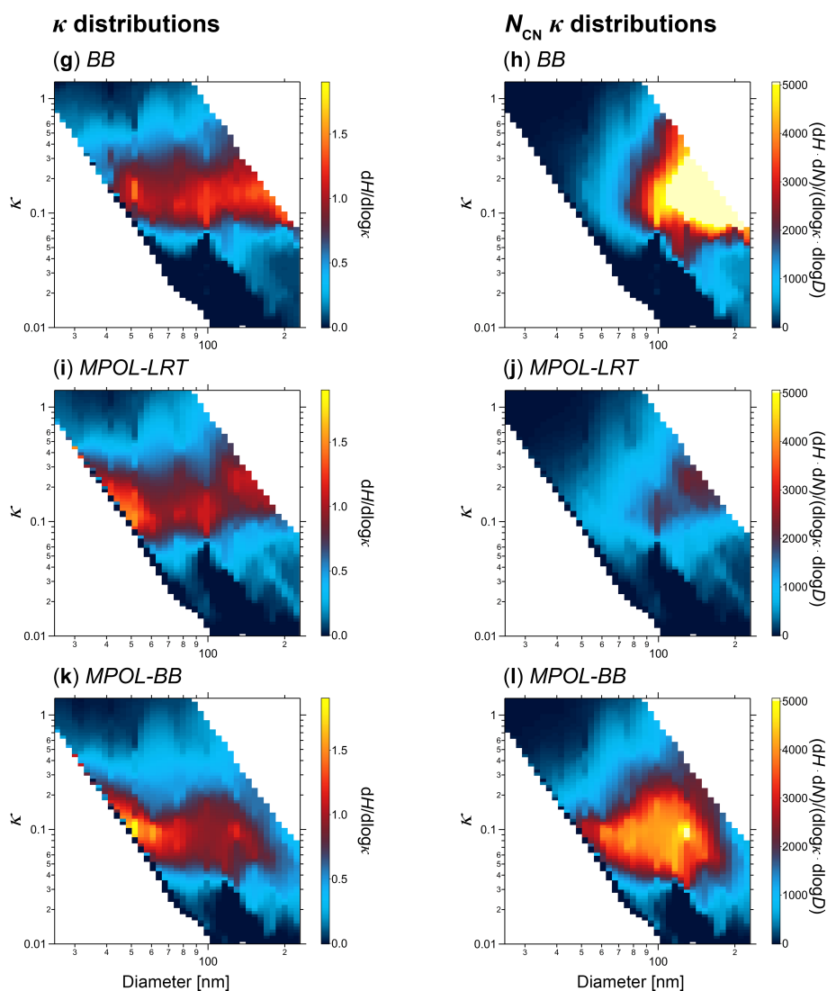
Figure 10. Average probability distribution of particle hygroscopicity, dH/d \log \kappa , on the left side and the same quantity weighted by the particle number size distribution, (dH \cdot dN)/(d \log \kappa \cdot d \log D) , on the right side, plotted over the effective hygroscopicity parameter, \kappa , and dry-particle diameter, D , for (a and b) the entire measurement period as well as (c and d) PR, (e and f) LRT, (g and h) BB, (i and j) MPOL-LRT, and (k and l) MPOL-BB conditions. The particle size distributions used for the weighting are shown in Fig. 6.
