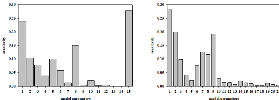
Fig. 3. Results of the FAST analysis for the (A) ethanol and nicotine (B) metabolism model
