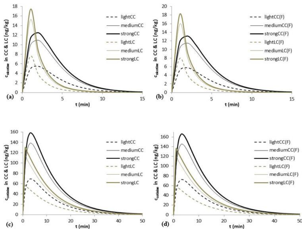
Fig. 2. Concentration profiles of nicotine models for male (a) and female (b) adolescents and cotinine model for male (c) and female adolescents (d) in two observed compartments; (i) central compartment (CC) and (ii) liver compartment (LC) based on the content of nicotine and cotinine in light, medium and strong cigarettes
