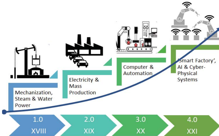
Figure 9: Industry 4.0.
