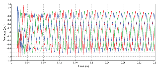
Figure 11 Transformer voltages at HV side during energization ( U_{\max} = 1,39 \text{ pu} )
