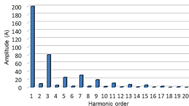
Figure 13 Frequency spectrum of the transformer inrush current in the phase A
