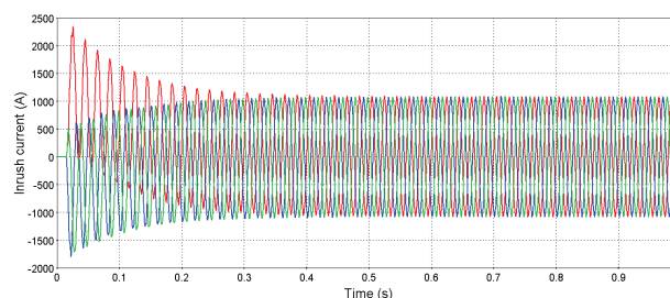
Figure 12 Transformer inrush currents ( I_{\max} = 4,85 \text{ pu} )
