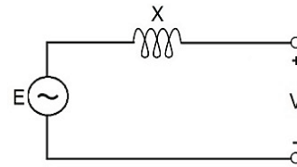
Figure 4 Representation of a generator as a constant voltage source behind transient reactance
