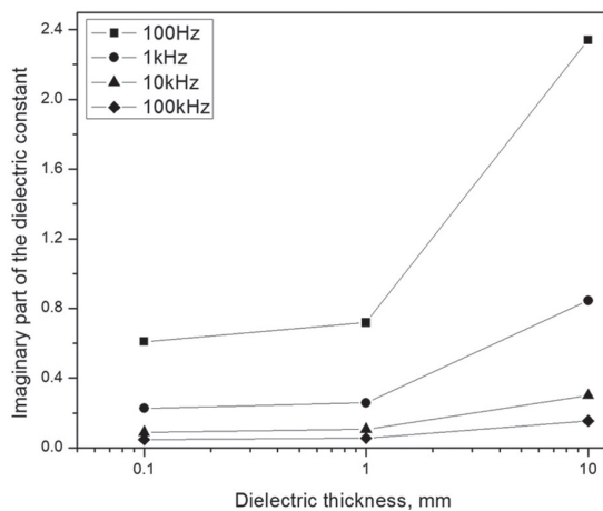
Fig. 8. A plot of the imaginary part of the dielectric constant versus the dielectric thickness for paper sheet with density 0.797 g/cm 3 at 21 o C calculated using equations (10) and (3) from measured values presented in Table 5.
