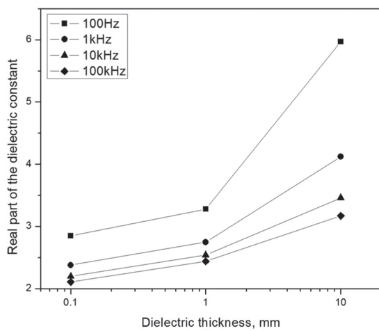
Fig. 7. A plot of the real part of the dielectric constant versus the dielectric thickness for paper sheet with density 0.797 g/cm 3 at 21 o C calculated using equations (10) and (3) from measured values presented in Table 5.
