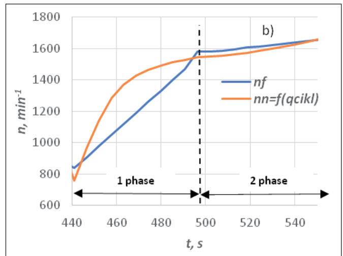
Fig. 8 Change in the Parameters of CAT3512B-HD DE Operation Mode in a Slow Acceleration Process
