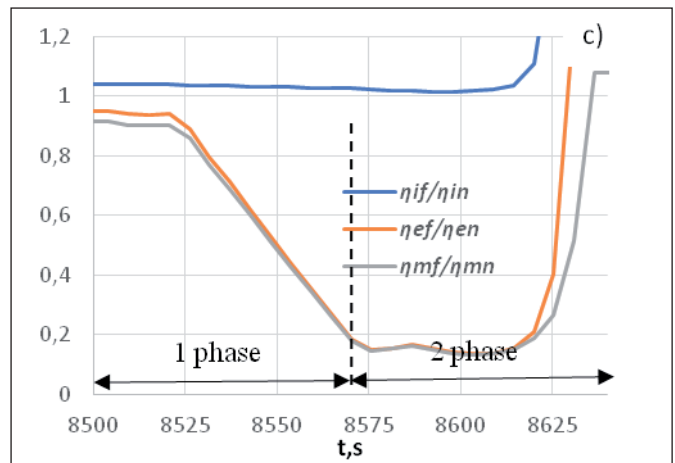
Fig. 11 Power Loss Transient Mode: a) – P_k , \alpha and q_{cycl} ; b) – Change in the Efficiency c) – Relative Efficiency.
