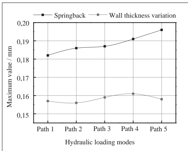
Figure 9 The effect of loading path on the formability of stamping
