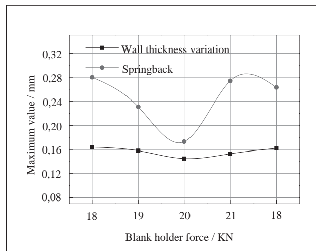
Figure 10 The effect of BHF on the formability of hydroforming part
