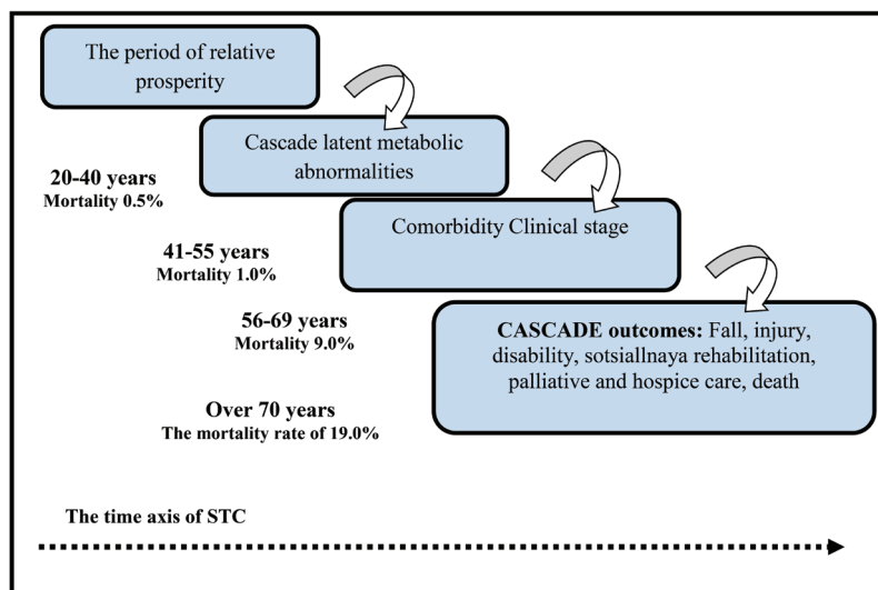
Fig. 3. Cascade mechanism of maladjustment to the effects of gravity.
