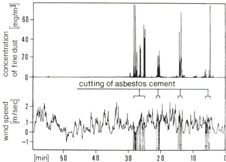
FIG. 1 - Time course of fine dust mass concentration on an open-air cutting place, where asbestos cement sheets are cut for a roof. The time constant of the TM-digital is 0.6 sec.
