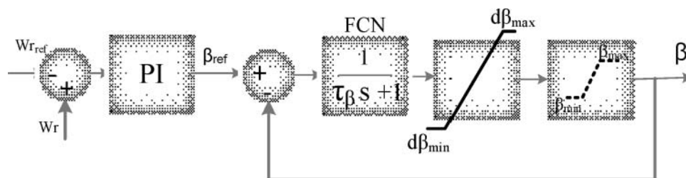
Figure 2. Block diagram of the pitch control system using PI controllers.
