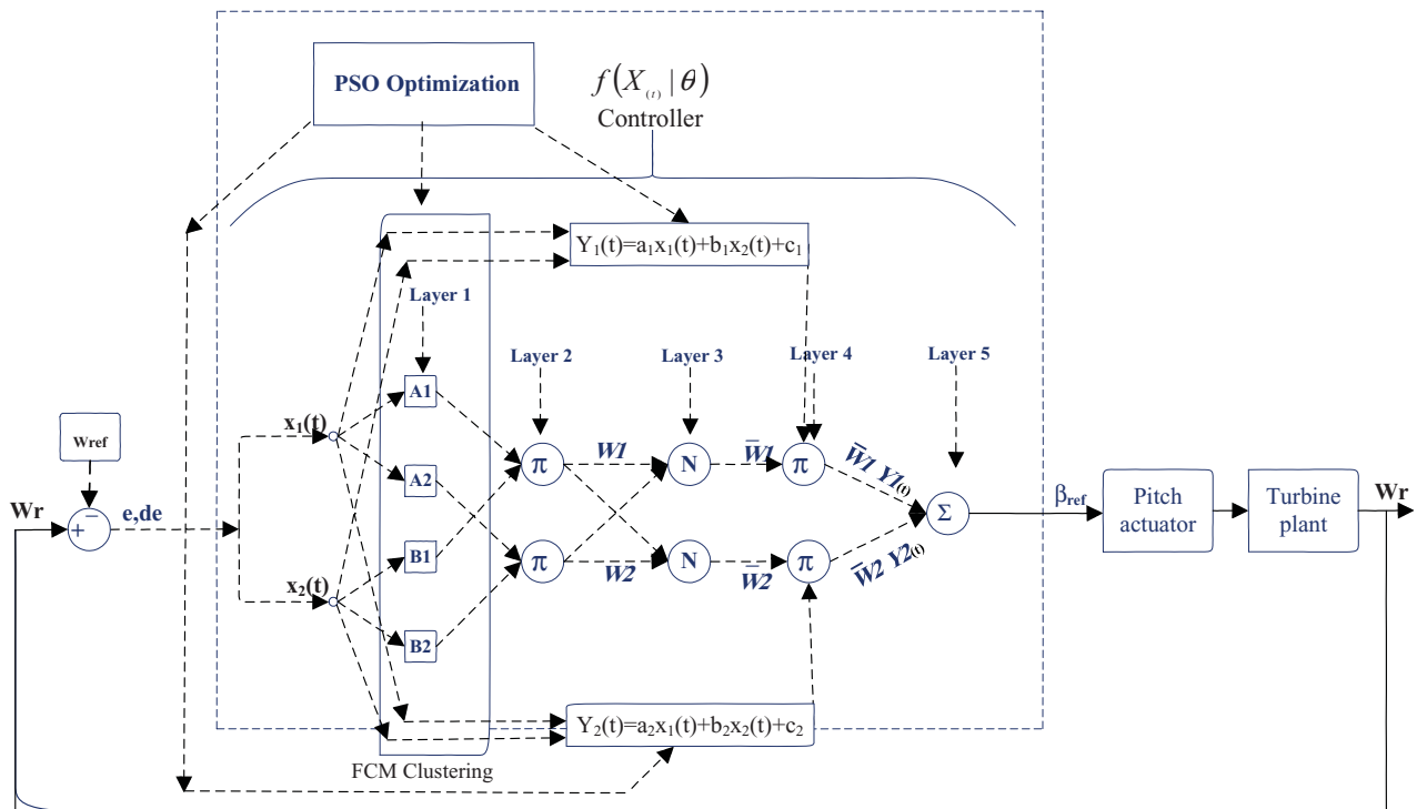
Figure 6. Structure of ANFIS 1 controller in proposed wind turbine.
