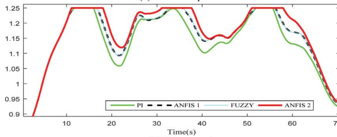
(c) Rotor speed
