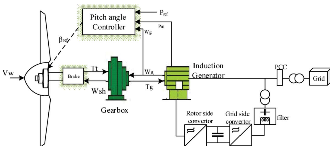
Figure 5. The block diagram of the fuzzy pitch angle controller.
