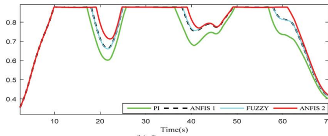
(b) Generator power
