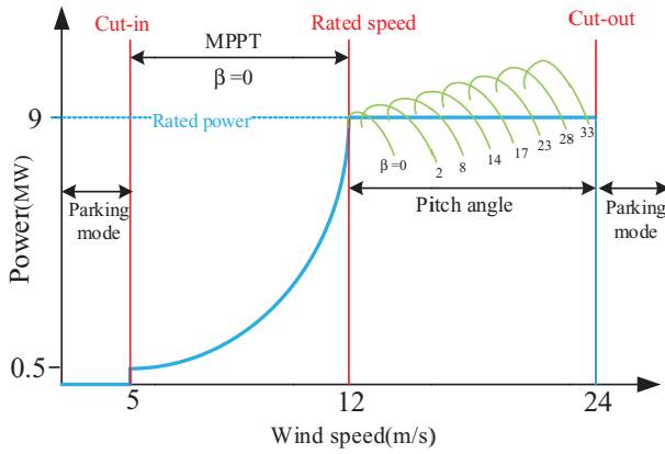
Figure 1. Qualitative wind turbine mechanical power versus wind speed curve.
