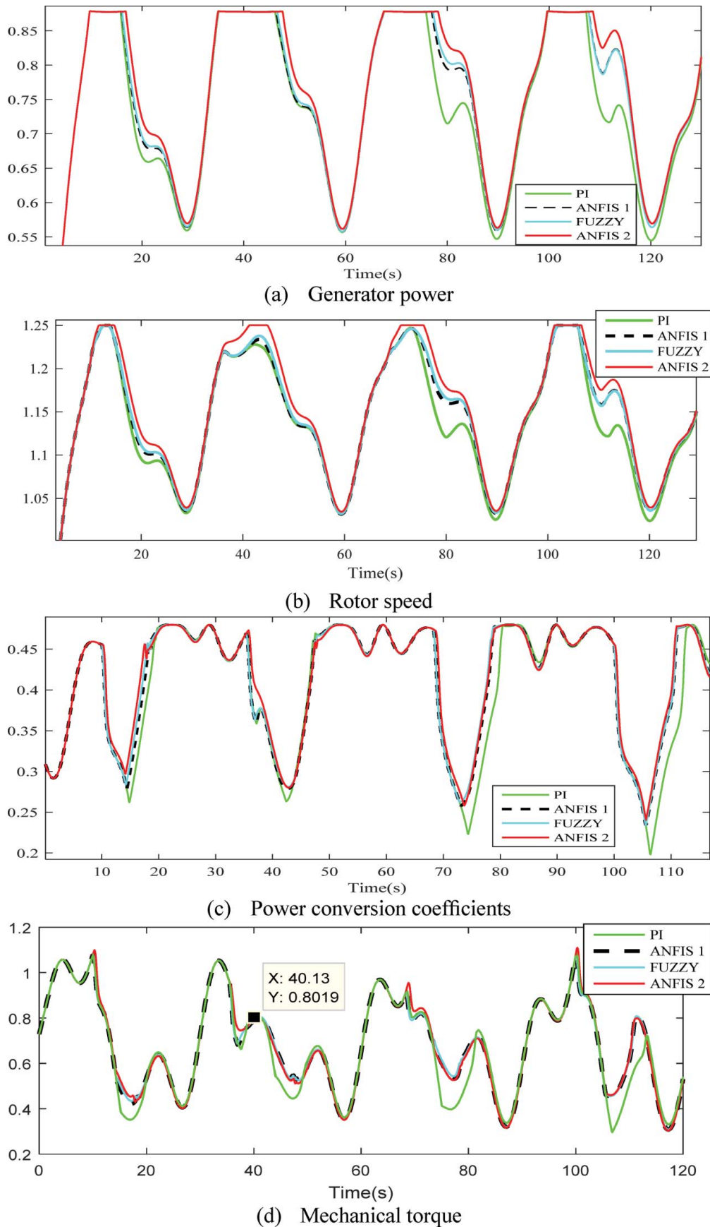
Figure 9. Simulation results for PI controller and proposed controllers at the mean wind speed of 13 m/s.
