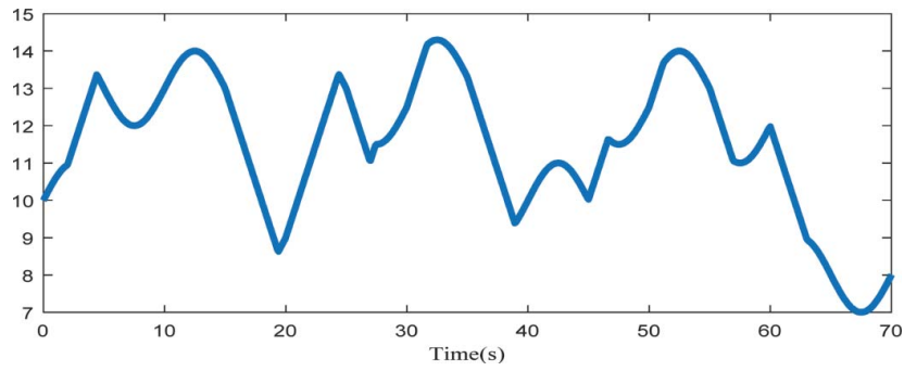
Figure 10. Pattern of realistic wind speed.
