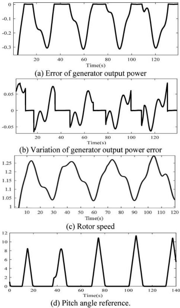
Figure 8. Control's signal of ANFIS 2 controller.
