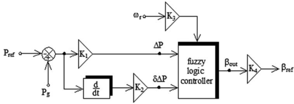
Figure 3. Block diagram of the FLC pitch angle control.
