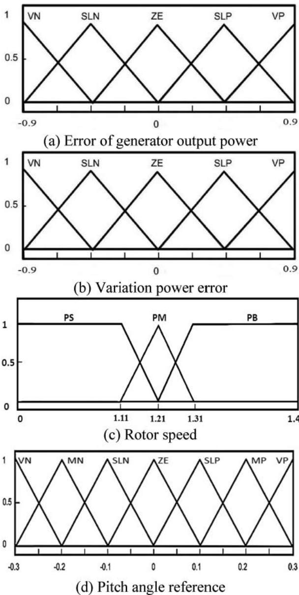
Figure 4. Membership functions of FLC.
