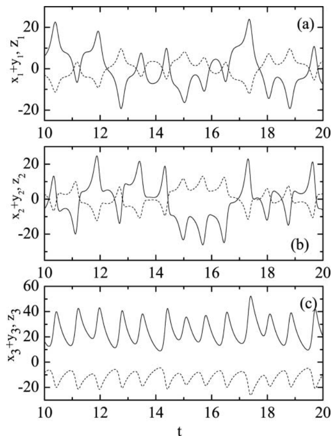
Figure 4. Combination projective synchronization between drive systems (5), (6) and response system (8) with \alpha = -2 . (a) Time waveforms of the states x_1 + y_1 (solid) and z_1 (dashed), (b) time waveforms of the states x_2 + y_2 (solid) and z_2 (dashed), (c) time waveforms of the states x_3 + y_3 (solid) and z_3 (dashed).
