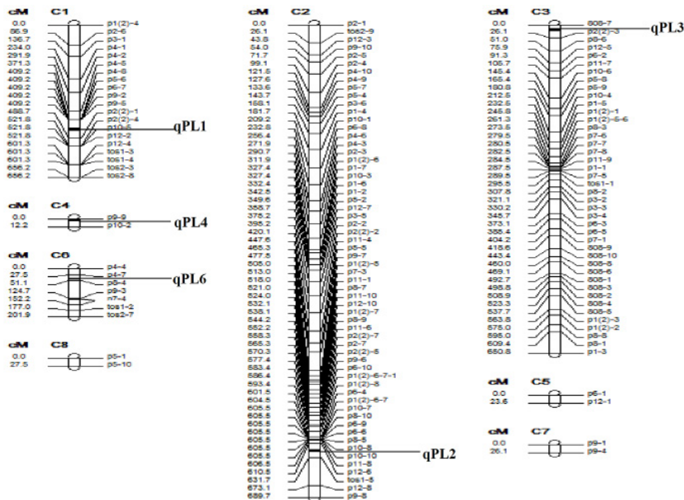
Figure 2. The chromosomal map and QTLs controlling plant height mapped in the F 2 : 3 population
