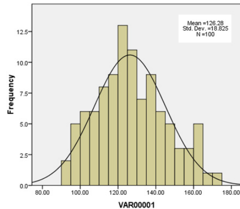
Figure 1. Frequency distribution of the means of the F 2:3 population for plant height
