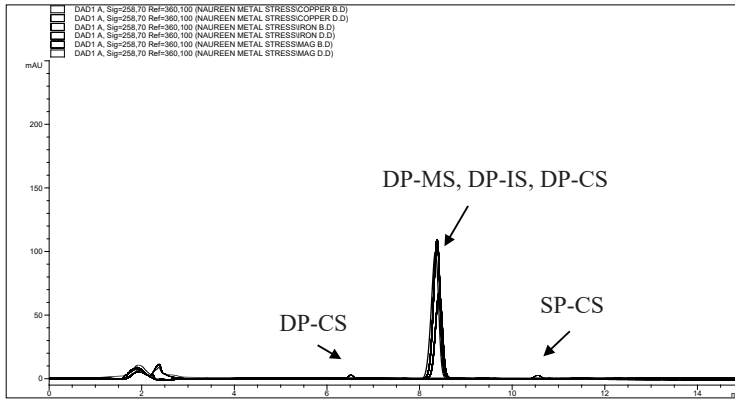
Fig. 6. Overlay of the chromatogram of OXCPM in 1.50 mmol L -1 stress solution of heavy metals (iron, copper, magnesium). SP – standard peak, DP-MS – degradation product in magnesium solution, DP-IS – degradation product in iron solution, DP-CS – degradation product in copper solution, SP-CS – standard peak in copper solution.
