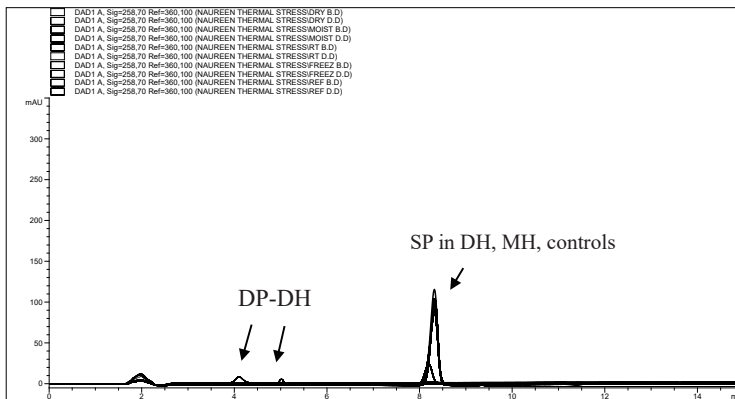
Fig. 7. Degradation behavior of OXCPM solution in dry heat. SP – standard peak, DP-DH – degradation product in dry heat at 150 ± 10 °C, MH – moist heat.
